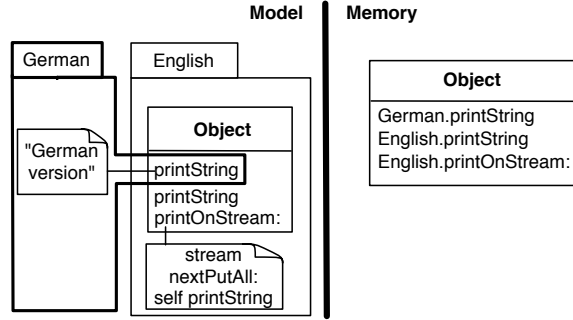
Figure 2: The class Object is composed of three methods: two versions of printString and a printOnStream: method.
