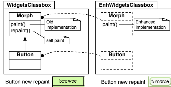
Figure 4: Implicitly rebinding classes within classboxes.
