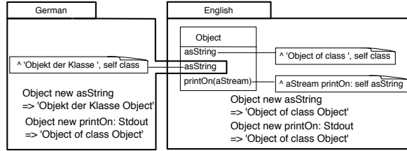
Figure 8: In Modular Smalltalk, namespace selectors are not reentrant: invoking printOn() from the German namespace does not invoke the German version of asString .
