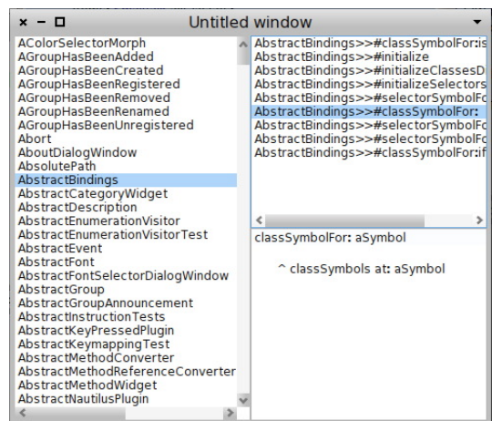
Figure 6. Classes browser
